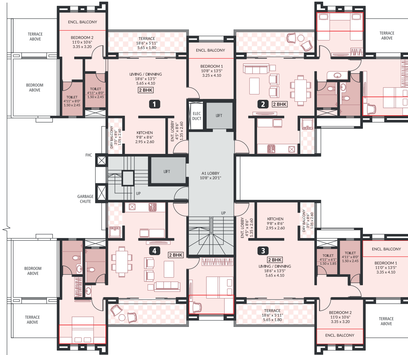
A1 WING - AREA STATEMENT - 1ST FLOOR (IN SQ.M/SQ.FT.)
