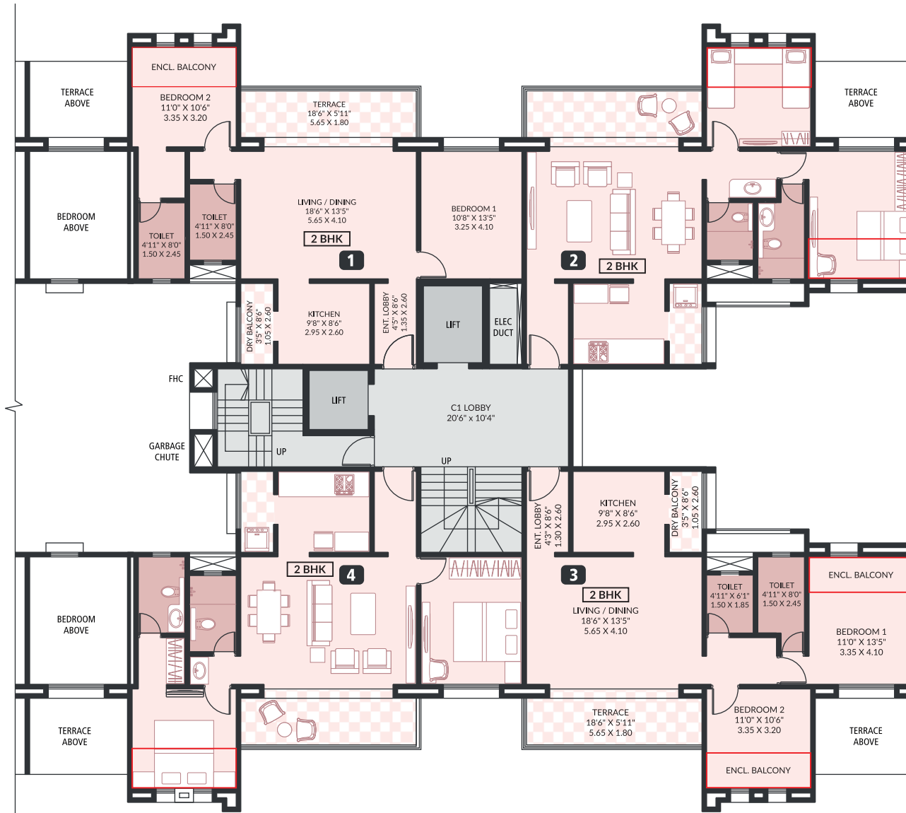
C1 WING - AREA STATEMENT - 1ST FLOOR (IN SQ.M/SQ.FT.)
