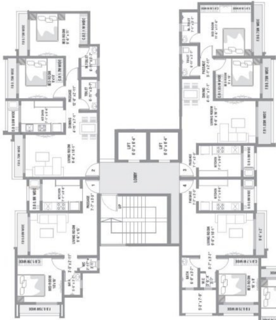
BLDG - 2 (PROPOSED)
