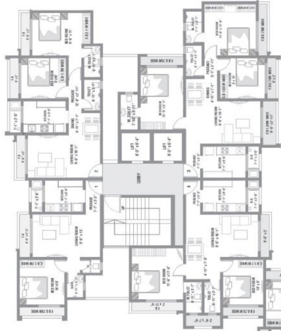
BLDG - 2 (PROPOSED)
